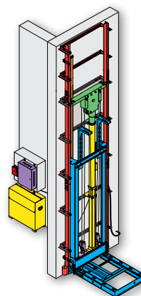
Excelelevator Roped Hydraulic Series 114 Capacity 1,000 lbs
