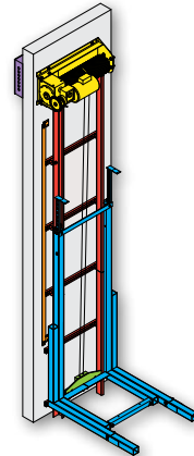
Paca-Glide, Winding Drum Machine Roomless Series 115 Capacity 1,000 lbs
